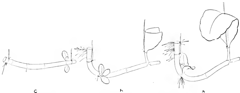
FIG. 104.—Same stems as in Fig. 102, 19 days later, May 29. Shoot in a greater than in b .
